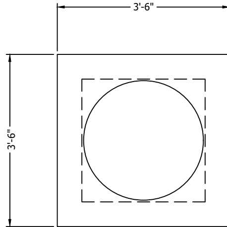
PLAN 1/2" = 1'-0"
