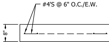
ELEVATION 1/2" = 1'-0"
