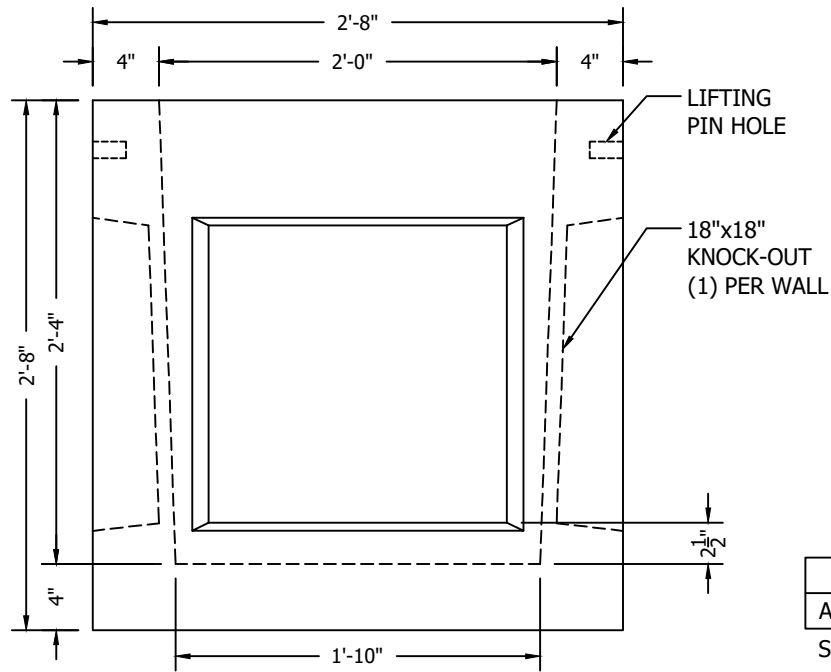
ELEVATION 1" = 1'-0"
