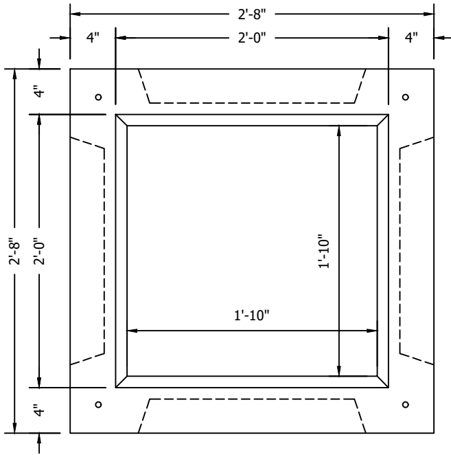
PLAN 1" = 1'-0"
