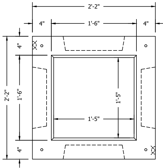
PLAN 1" = 1'-0"
