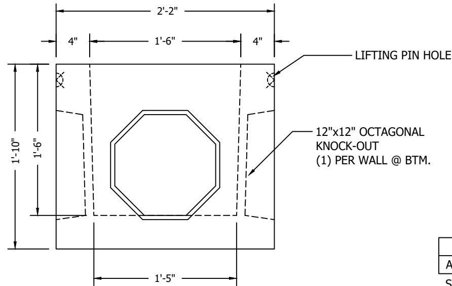
ELEVATION 1" = 1'-0"
