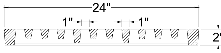
SECTION B-B
